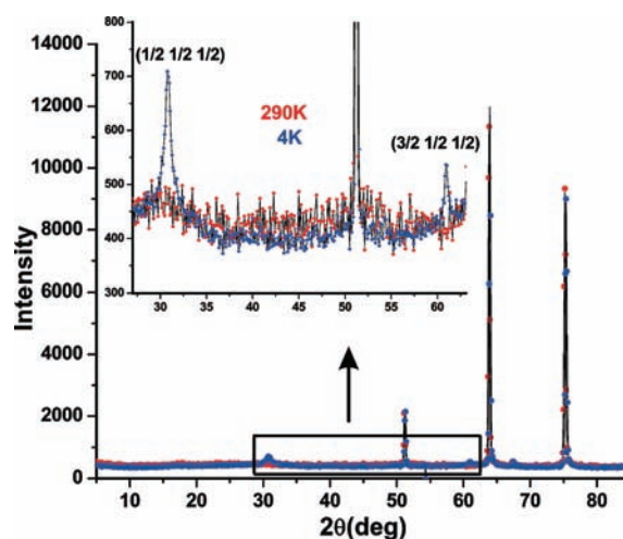
Figure 12. Neutron diffraction data for \text{Sr}_2\text{FeMnO}_{5.0}(\text{Ar}) at 4 K (blue) compared with data at 290 K (red), showing the presence of broad magnetic features at \sim 31^\circ and 61^\circ that can be indexed as (\frac{1}{2} \frac{1}{2} \frac{1}{2}) and (\frac{3}{2} \frac{1}{2} \frac{1}{2}) on the primitive cubic cell, indicative of short-range G-type magnetic order (inset).
